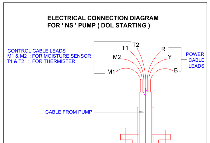
Figure (3): DOL-connection
